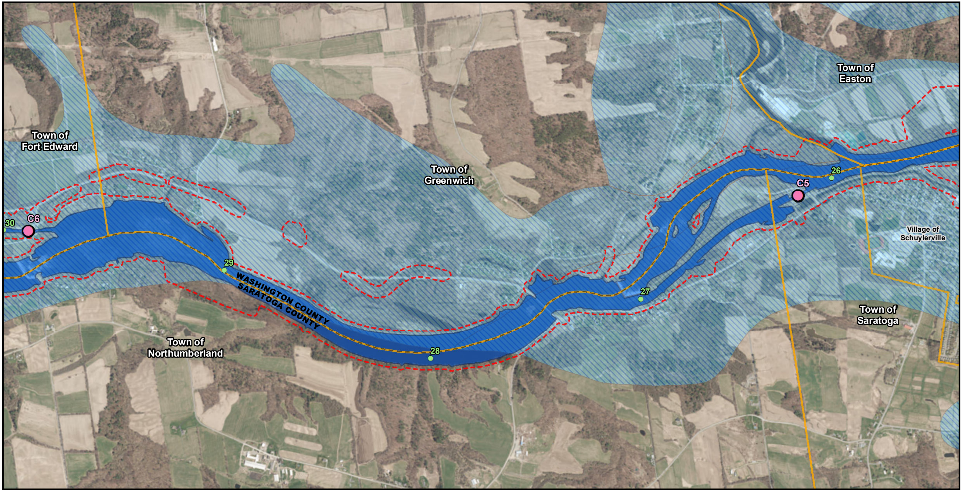
Figure 10F: Aquifers
